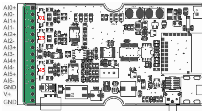
012345: For AI0/1/2/3/4/5 Select Current Input (ON Position) Voltage Input (OFF Position)
