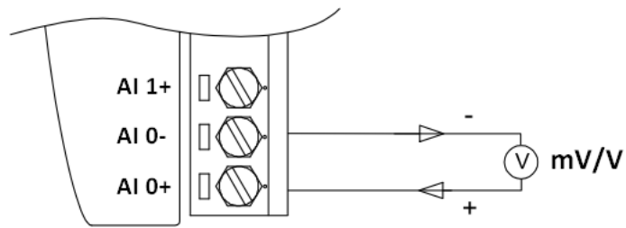
Figure 3.2 Voltage Input Wiring Diagram of ADAM-2017PZ
