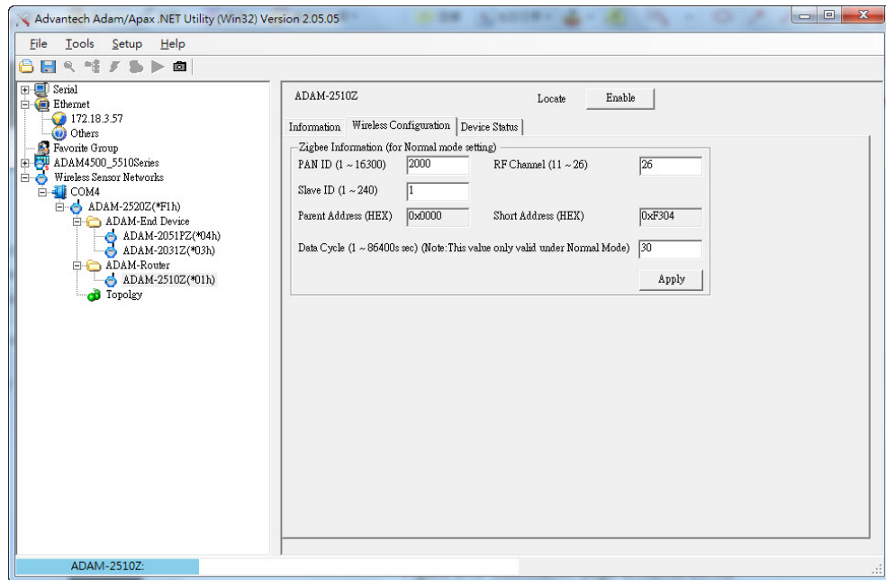
Figure 5.14 Wireless Configuration page of ADAM-2510Z
