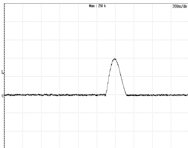
Figure 11: Inrush current @ Vin=72V CH1:lin, 2A/div, 20ns/div; Max current 4A, I_2t=1.7E-7A^2S
