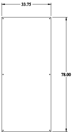
INNER PANEL
